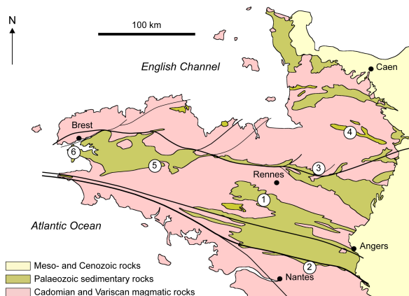
Fig. 1. Simplified geological map of the Armorican Massif (western France) showing the six main areas yielding Darrivilian stylophorans; 1, Martigné Ferchaud Syncline (Traveusot Formation); 2, Ancenis Syncline (Pierre Meslière Formation); 3, Menez-Belair Syncline (Andouillé Formation); 4, Mortain-Domfront Syncline (Le Pissot Formation); 5, eastern part of the Châteaulin Basin (Postolonnec Formation); 6, Crozon Peninsula (Postolonnec Formation).
